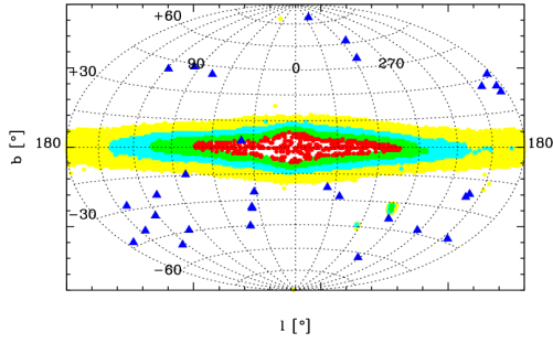
Fig. 1. Whole sky Aitoff projection showing in Galactic coordinates the positions of the 31 cPOCRs (triangles). 2MASS background stellar densities are shown in five levels, corresponding to the 20th, 40th, 60th and 80th percentiles in the \log(\rho_{field}) distribution, considering star counts with K_s < 14 mag per square degree.
