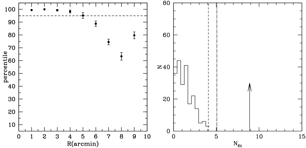
Fig. 5. Left Panel: Search of the optimal object radius. The horizontal dashed line indicates the 95th percentile locus. Right Panel: Field samplings of stars that fit an isochrone weighted by membership probability; the POCR counterpart is indicated by the arrow. We conclude that Renou 38 is very distinct from the surrounding fields.
