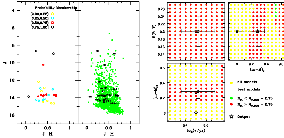
Fig. 6. Same as Fig. 4 but for NGC 843 ( R=5' ). The NGC 843 is indistinguishable from the surrounding fields.
