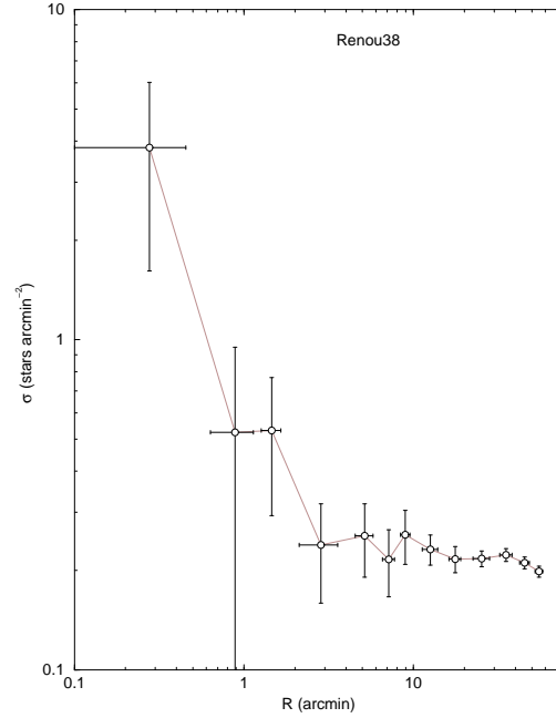
Fig. 3. Renou 38 stellar RDP provide a general view of POCR structure. Poisson errors are also shown.
