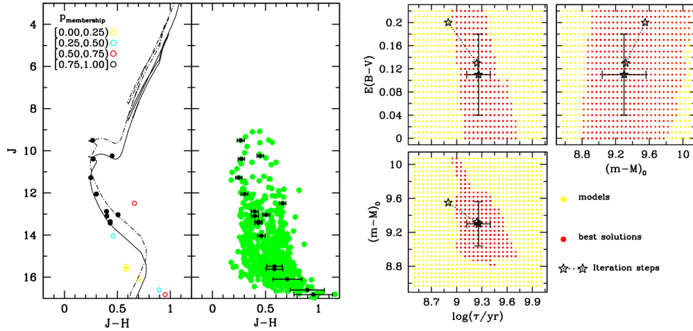
Fig. 4. Left Panel: Renou 38 J \times (J-H) CMD where membership probabilities are shown in colour code. Solar metallicity isochrone, together with shifted one due to binaries of equal masses (dashed line). The POCR stars ( R=4' ) are plotted over the control field in green ( R=30' ). Right Panel: Parameter space where the evolution of the output solution (open star) is shown.
